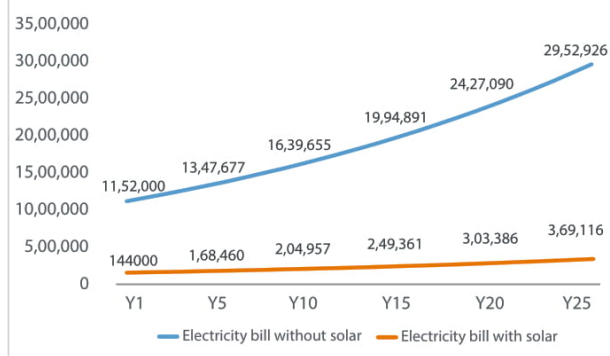
Typical Electricity Bill Comparison with and without Solar 3 (Rs.)
